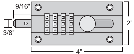
Bolt Receiver for Flush Mounting
